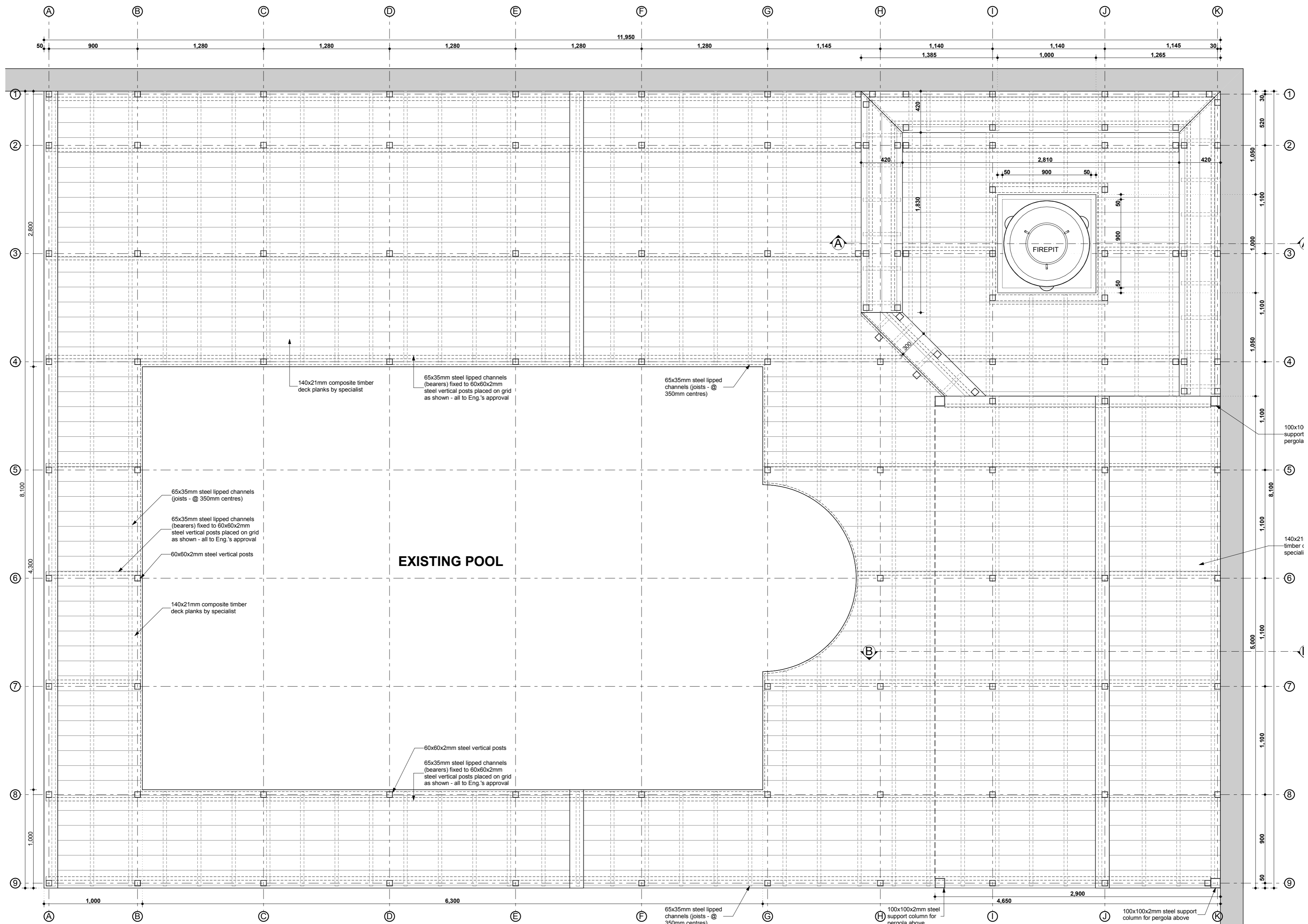
TIMBER DECK LAYOUT PLAN SCALE 1:25
